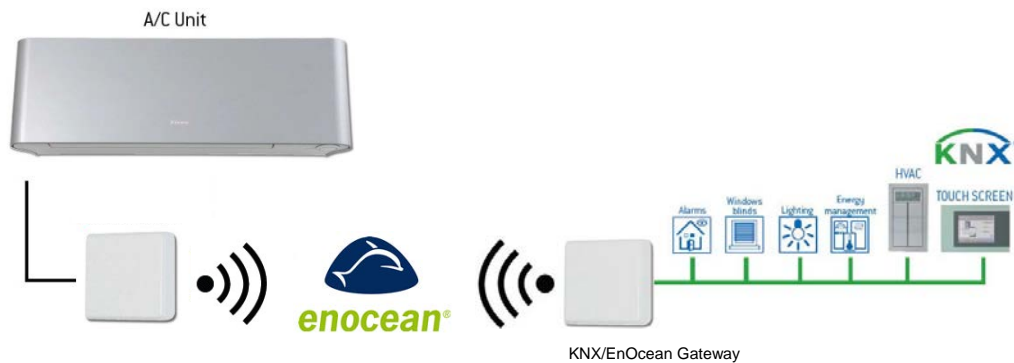
Figure 3.1 KNX/EnOcean Gateway and EnOcean Air Conditioner integration example
