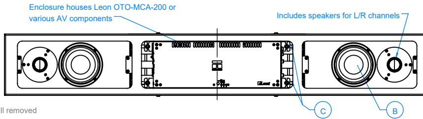
Front View with grill removed
