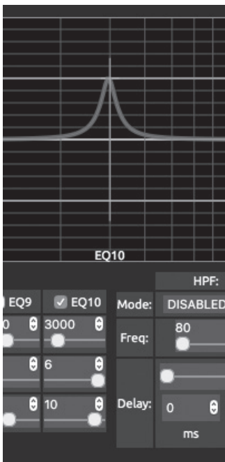
Figure 13. 3kHz center frequency, Q=6, 10dB gain
